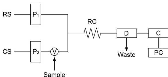
Fig. 1. FIA system for the determination of ascorbic acid. RS: 1 \mu\text{mol L}^{-1} perylenebisimide-linked nitroxide (reagent) solution in 20 \text{ mmol L}^{-1} HCl/THF (1/1, v/v); CS: carrier solution of 20 \text{ mmol L}^{-1} HCl/THF (1/1, v/v); P 1 , P 2 : pumps; V: injector with sample loop ( 100 \mu\text{L} ); RC: reaction coil ( 0.50 \text{ mm} , i.d.); D: fluorescence detector; C: A/D converter; PC: computer.
