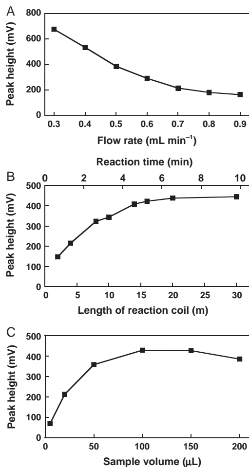
Fig. 3. Optimization of flow conditions for the determination of ascorbic acid. (A) Effect of flow rate, coil length: 10 m; sample volume: 50 μL. (B) Effect of reaction coil length, flow rate: 0.5 mL min -1 ; sample volume: 50 μL. (C) Effect of sample volume, coil length: 10 m, flow rate: 0.5 mL min -1 . Concentration of ascorbic acid was 4.0 μmol L -1 . RS and CS are the same as in Fig. 1.
