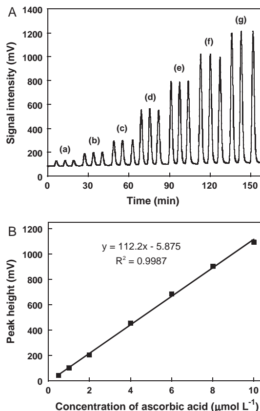
Fig. 4. (A) Flow signals for the determination of ascorbic acid. Concentration of the standard solution of ascorbic acid; (a) 0.5 μmol L -1 , (b) 1.0 μmol L -1 , (c) 2.0 μmol L -1 , (d) 4.0 μmol L -1 , (e) 6.0 μmol L -1 , (f) 8.0 μmol L -1 , (g) 10.0 μmol L -1 . Flow condition; flow rate: 0.5 mL min -1 ; sample volume: 100 μL, reaction coil length: 20 m. (B) Calibration curve for the determination of ascorbic acid. RS and CS are the same as in Fig. 1.
