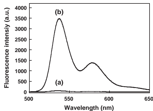
Fig. 2. Fluorescence spectra of the perylenebisimide-linked nitroxide (PBILN) ( 1 \mu\text{mol L}^{-1} ) in 20 \text{ mmol L}^{-1} HCl/THF (1/1, v/v) solution with excitation at 490 \text{ nm} . (A) Fluorescence spectrum of PBILN before the addition of ascorbic acid, (B) fluorescence spectra of PBILN after the addition of an ascorbic acid solution ( 100 \mu\text{mol L}^{-1} ).
